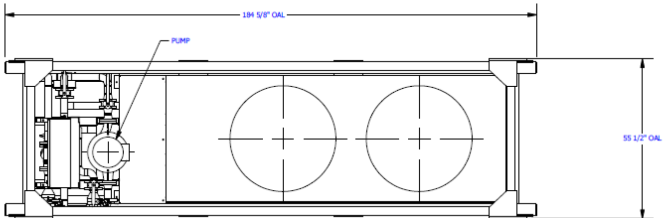
Plan View with Dimensional Data
