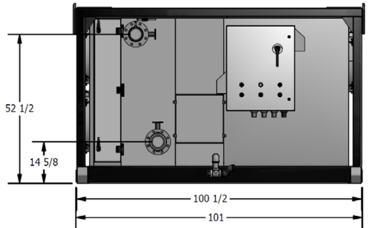
Chilled Water & Electrical Connections with Dimensional Data
