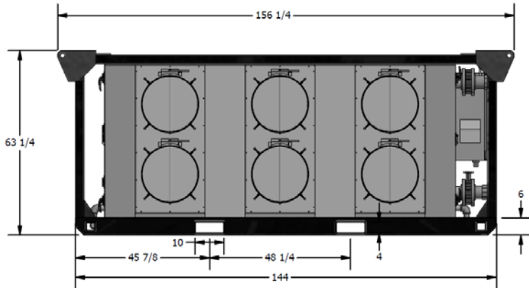
Six (6) 20" Return Air Connections
