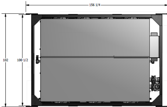
Plan View with Dimensional Data
