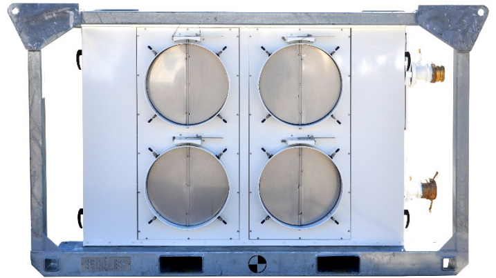
Four (4) 20" Return Air Connections
